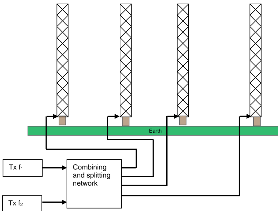
Example 7: multi-mast arrays. For example, Langley Mill, four masts on two frequencies.
